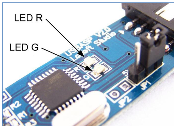
Figure 3. LEDs
