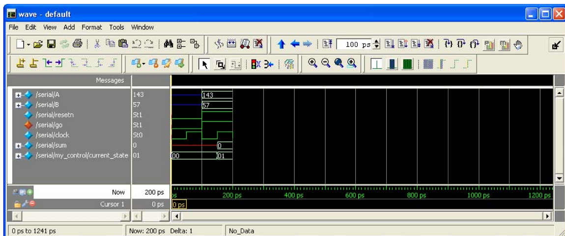
Figure 21. Simulation results after 200ps.
