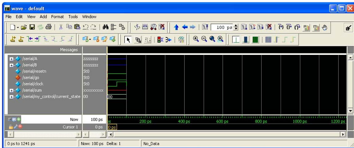
Figure 19. Simulation results after 100ps.
