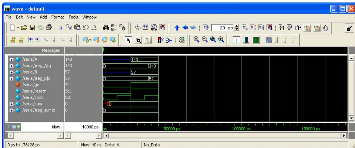
Figure 28. Timing Simulation after 40ns.
