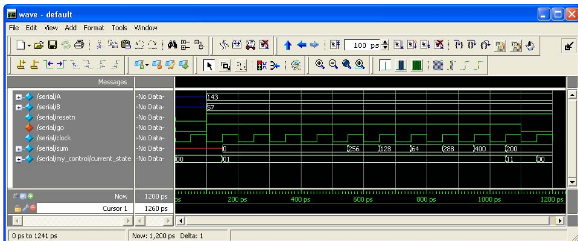
Figure 23. Simulation results after 1200ps.
