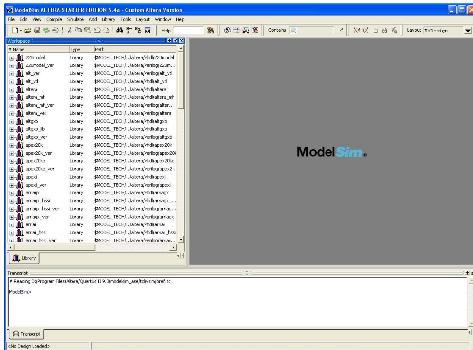
Figure 7. ModelSim window.
