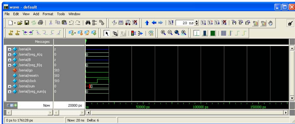
Figure 27. Timing Simulation after 20ns.
