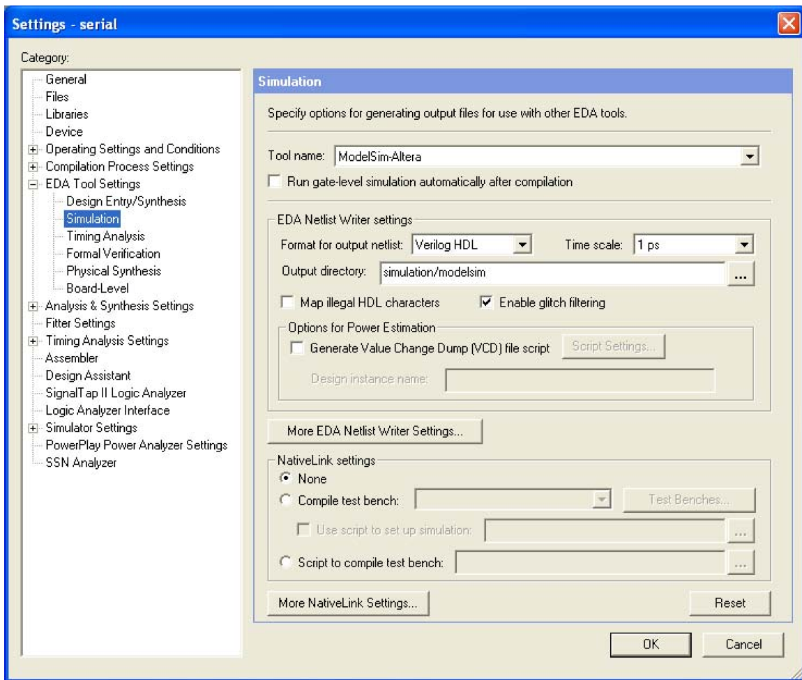
Figure 24. Quartus II EDA simulation tool settings.
