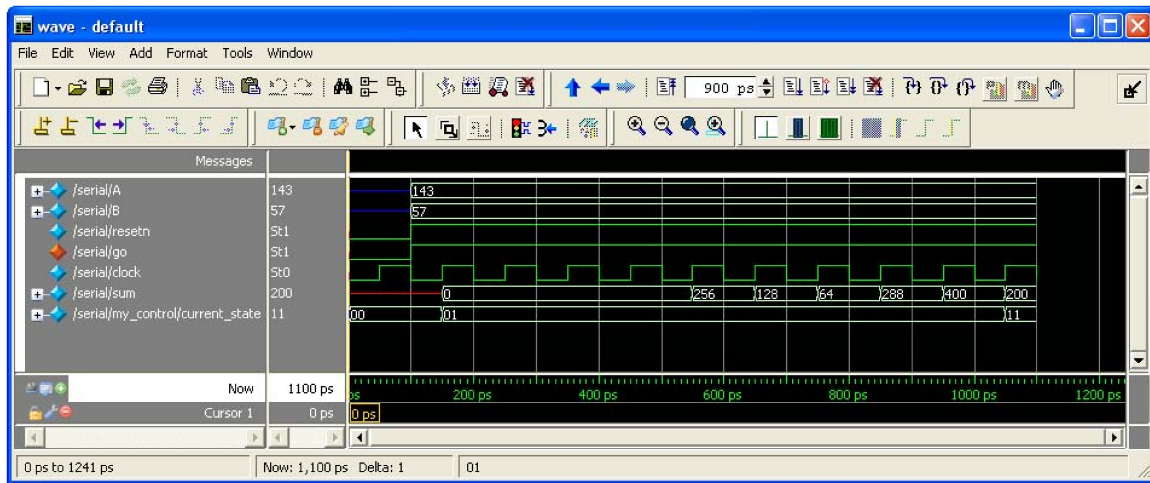
Figure 22. Simulation results after 1100ps.
