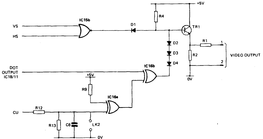
Figure 16. Video Output Circuit
