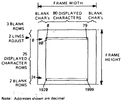
Figure 2. VDU Scan (1 Frame 50Hz)
