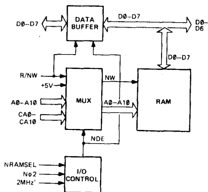
Figure 12. Character RAM Circuit
