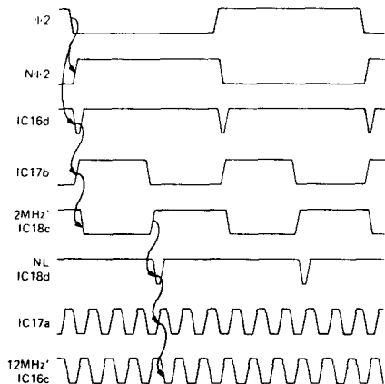
Figure 11. VDU Clock Timing ( \Phi 2 = 1\text{MHz} )
