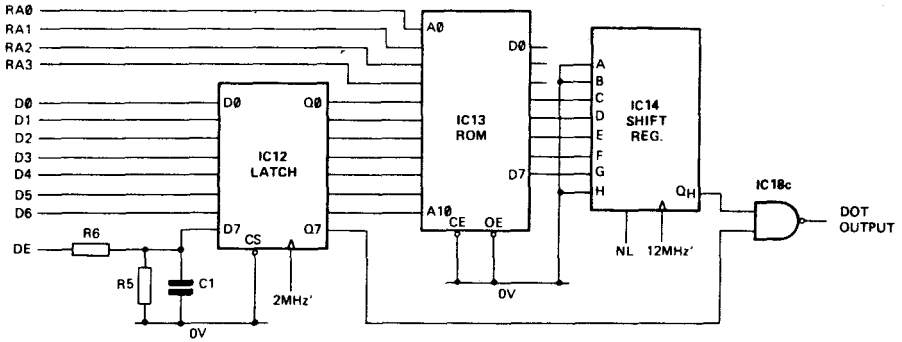
Figure 14. Character Generator Circuit
