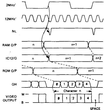
Figure 15. Character Generator Timing
