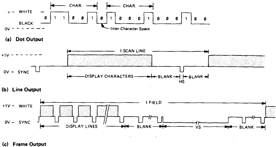
Figure 17. Composite Video Output Signal
