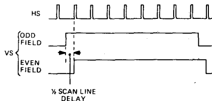
Figure 9. VS Signal Timing Interlace-Sync Mode
