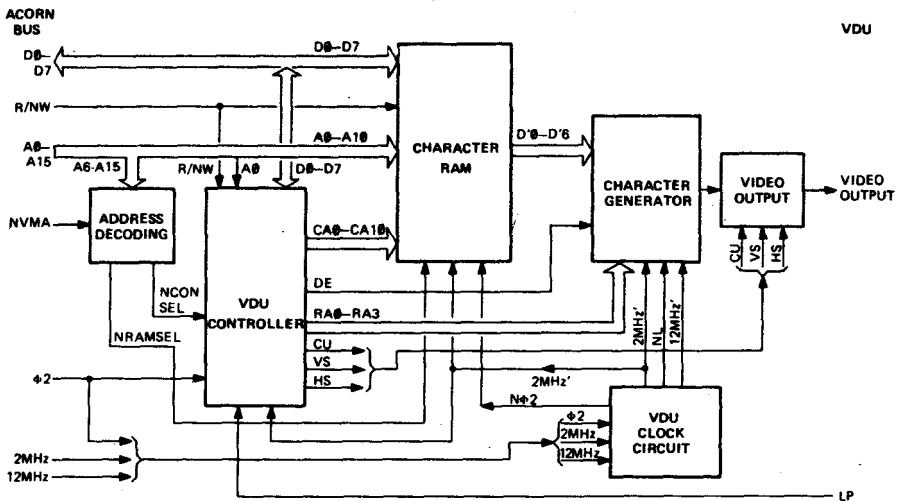
Figure 1. 80 x 25 VDU Interface Board Block Diagram
