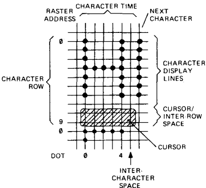
Figure 3. Character Dot Matrix
